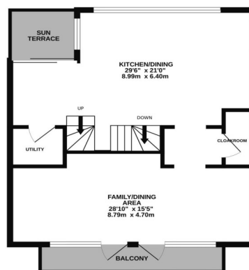
1ST FLOOR
